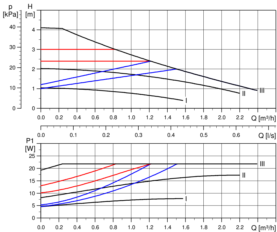
Fig. 16 Curbe caracteristice, ALPHA2 L XX-40
