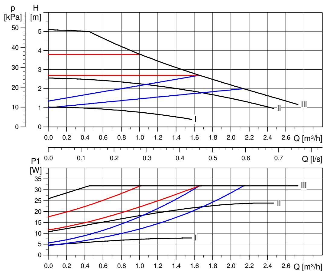
Fig. 17 Curbe caracteristice, ALPHA2 L XX-50
