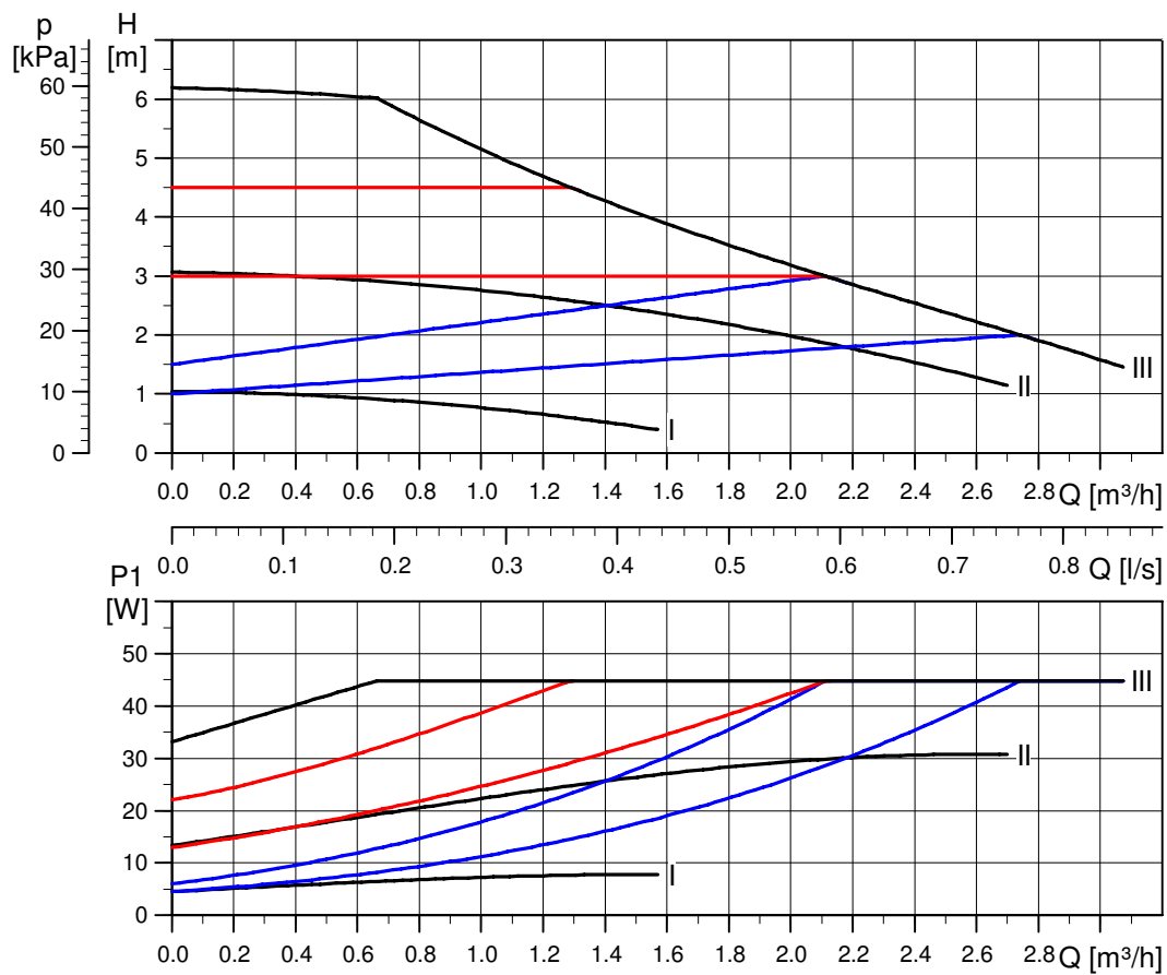
Fig. 18 Curbe caracteristice, ALPHA2 L XX-60
