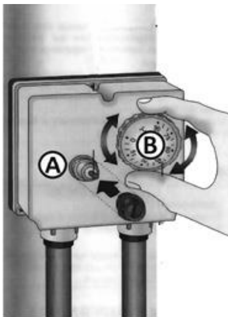
scheme 8
