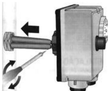
scheme 4
