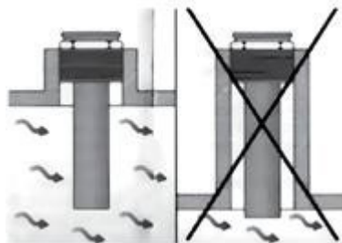
scheme 6
